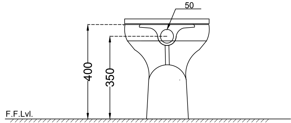
BACK VIEW
